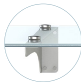
Bracket System „L” glass canopy on a bracket with the cross-section „L”, cutout type „Triangle”
