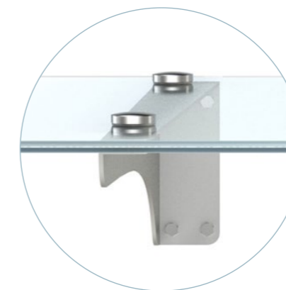
Bracket System „L” glass canoping on a bracket with the cross-section „L”
