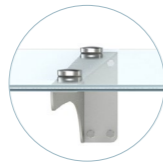
Bracket System „L” glass canopy on a bracket with the cross-section „L”, cutout type „Slim”
